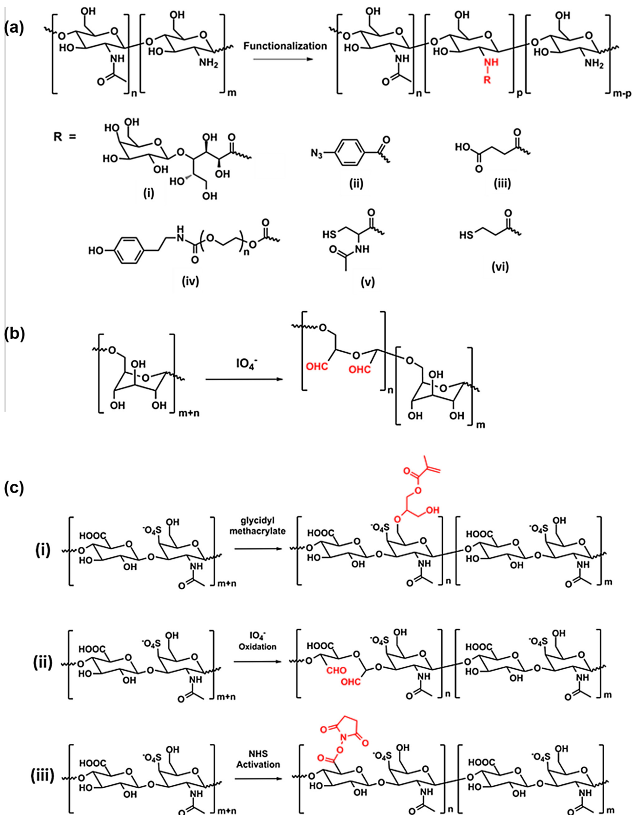
Fig. 3. Representative chemical structures of polysaccharide-based sealants. (a) Deacetylation of chitin generates chitosan with different degrees of acetylation, and various chemically modified chitosan derivatives are obtained by reacting chitosan with (i) lactobionic acid, (ii) 4-azidobenzoic acid, (iii) succinic anhydride, (iv) PEG oligomers, (v) N -acetylcysteine, and (vi) 3-mercaptopropionic acid at the amine site [51–57]. (b) Preparation of aldehyde-containing dextran via selective partial oxidation by periodate [60,61]. (c) Chemical modification of chondroitin sulfate to introduce (i) methacrylate groups via reacting with glycidyl methacrylate [63], (ii) aldehyde groups via the oxidation reaction by periodate [64], and (iii) NHS-activated ester groups [66].
